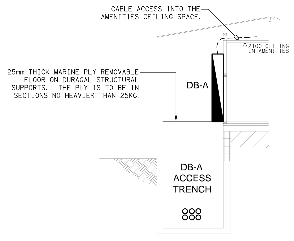
DETAIL B DB-A ACCESS TRENCH SECTION SCALE 1:50
